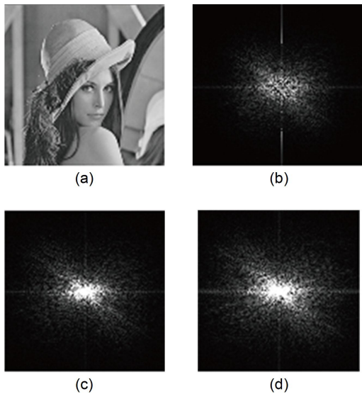
Fig. 6 The original image (a) and the frequency spectrum maps with FFT (b), CFT (c), and SFCFT (d)
